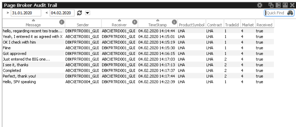
Fig. 85: Screenshot of the Page Broker Audit Trail view showing TES messages
