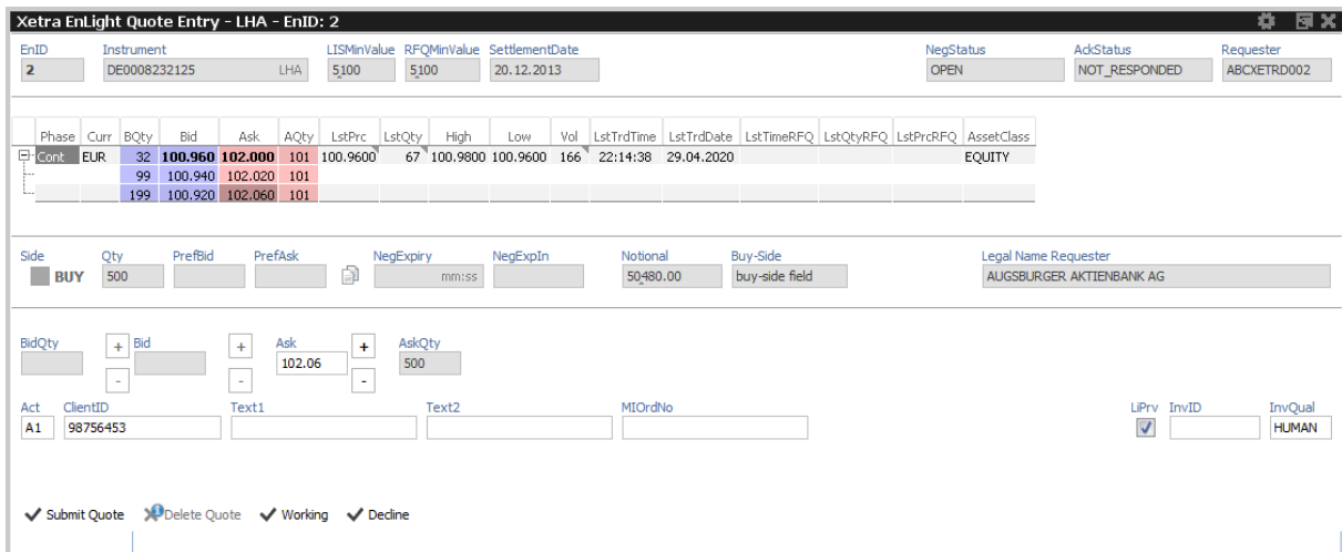
Fig. 74: Screenshot of the Xetra EnLight Quote Entry view
