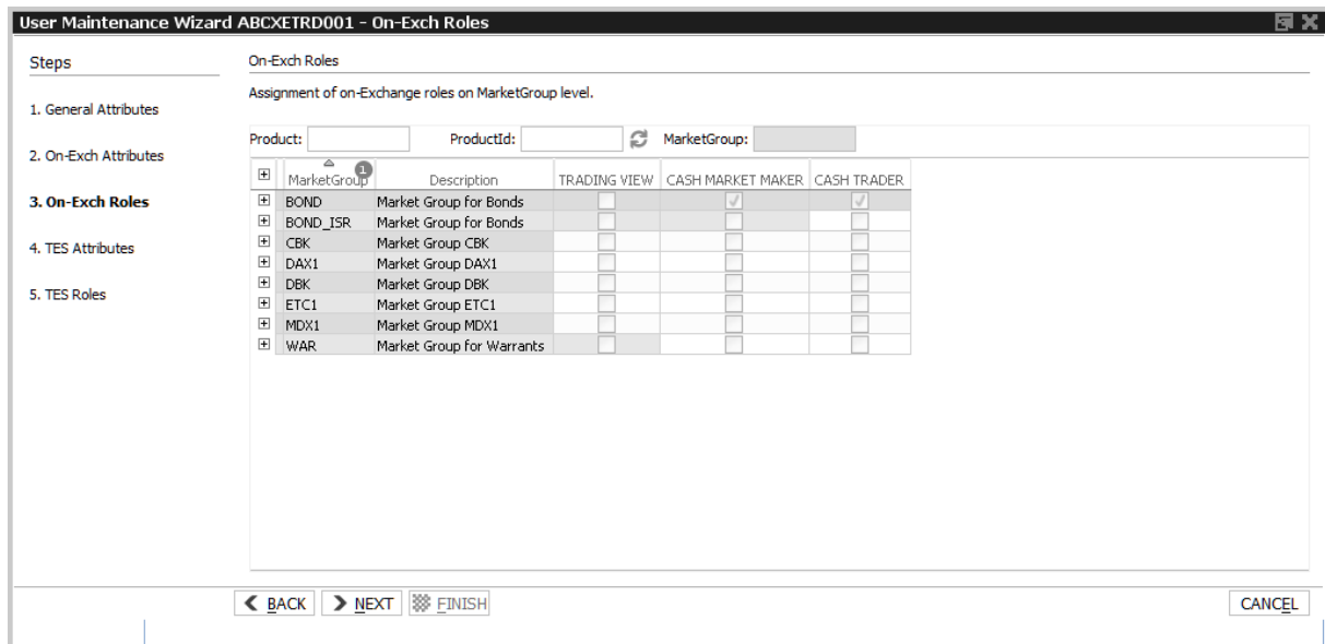
Fig. 94: Screenshot of the User Maintenance Wizard showing the entitlement roles on the On-Exch Roles tab
