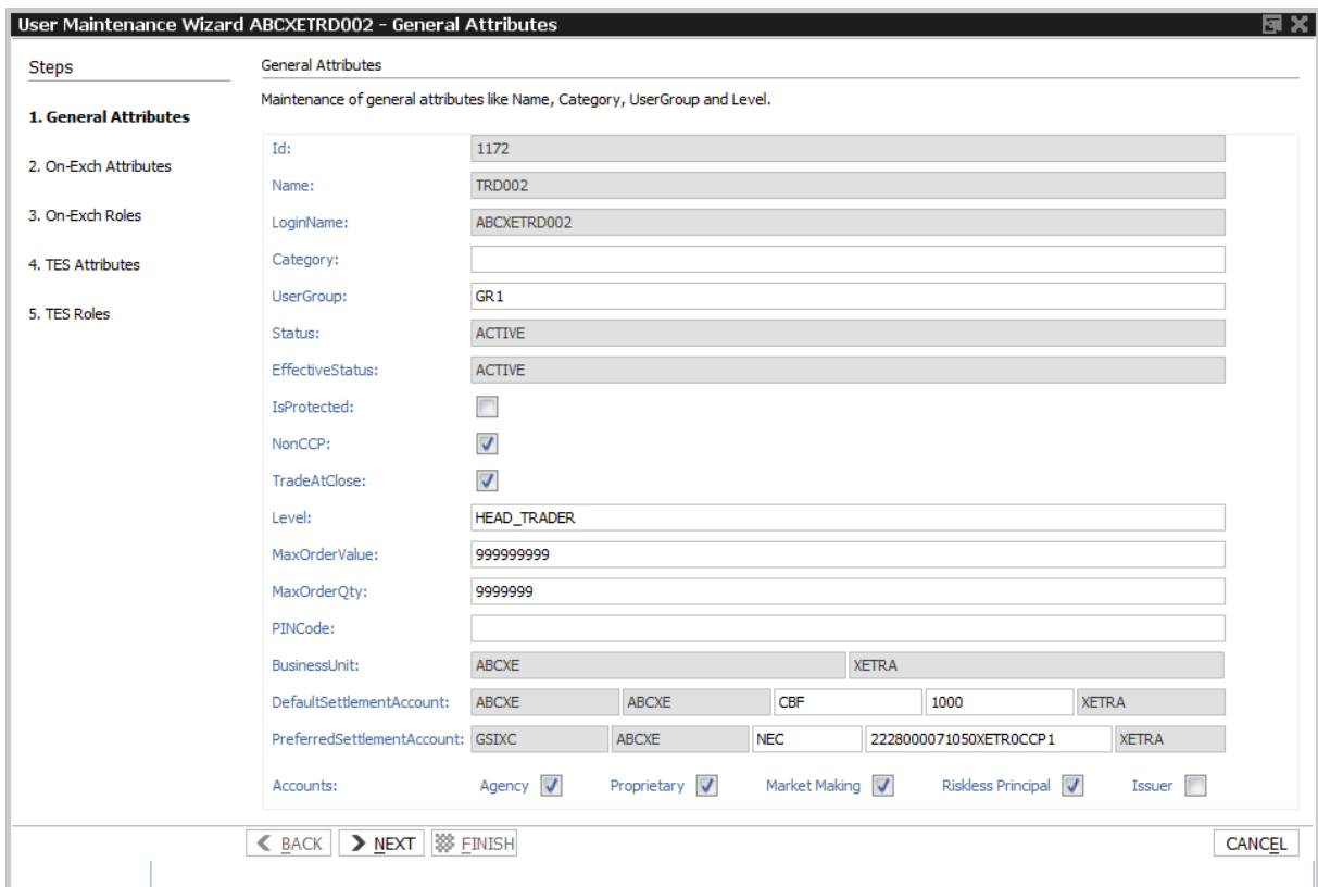
Fig. 89: Screenshot of the User Maintenance Wizard showing the General Attributes tab
