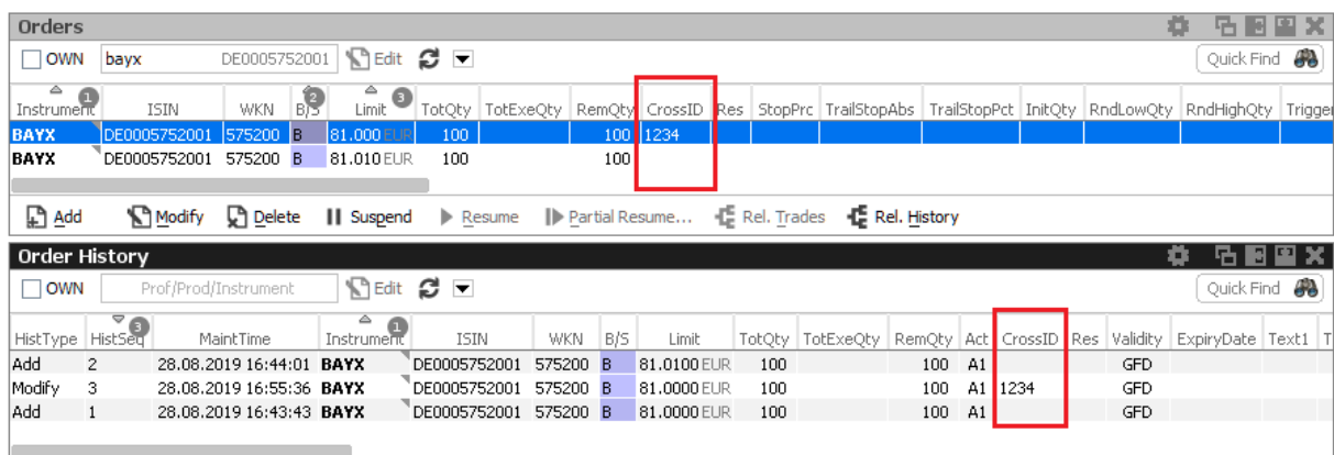
Fig. 58: Screenshots showing the CrossID column of the Orders and Order History view
