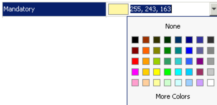
Fig. 16: Color Chooser
