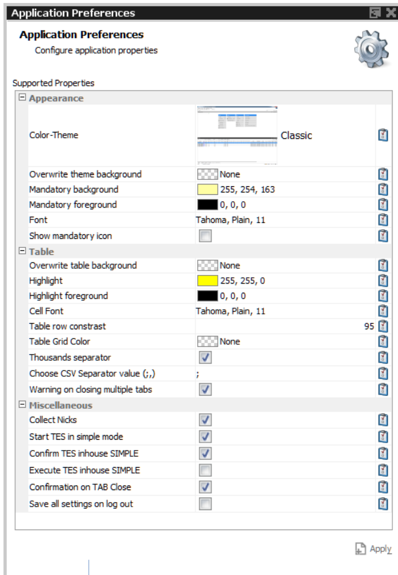
Fig. 42: Application Preferences view
